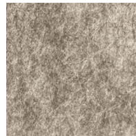
TUFF
