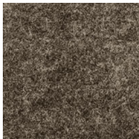
NORITE
