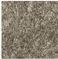
GNEISS
